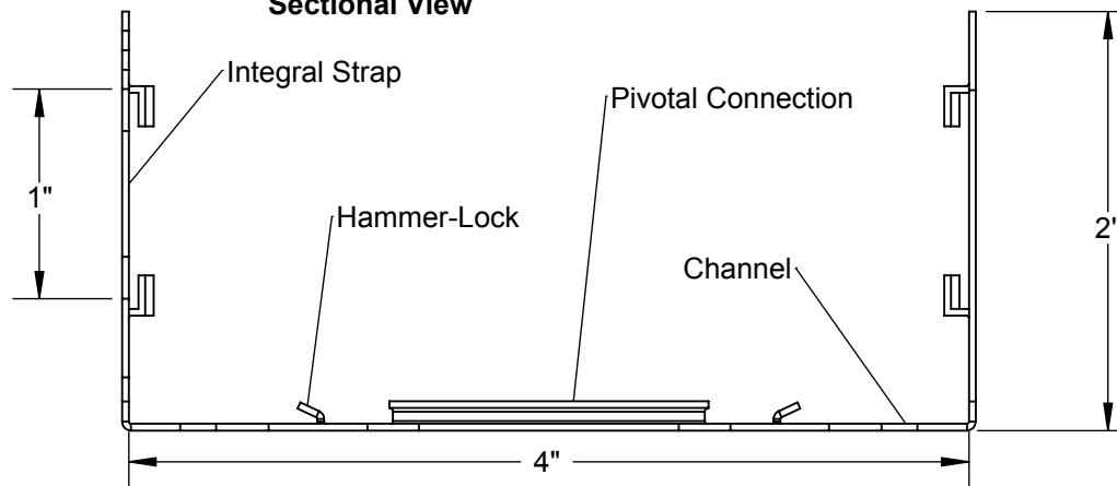
Sectional View
