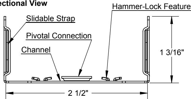
Sectional View
