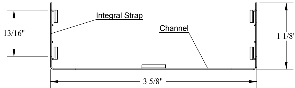
Sectional View
