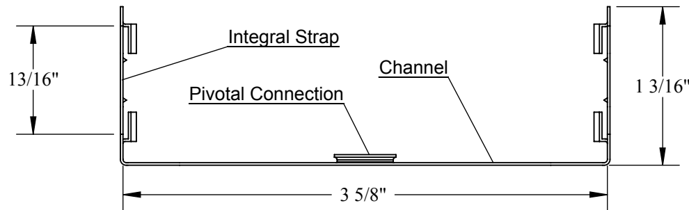
Sectional View
