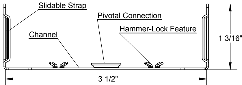
Sectional View
