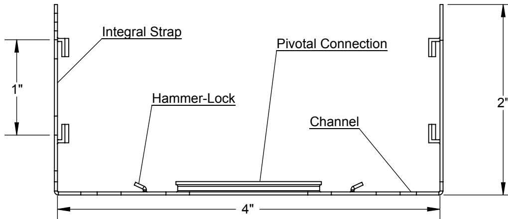
Sectional View
