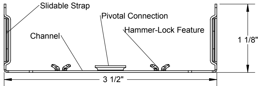
Sectional View
